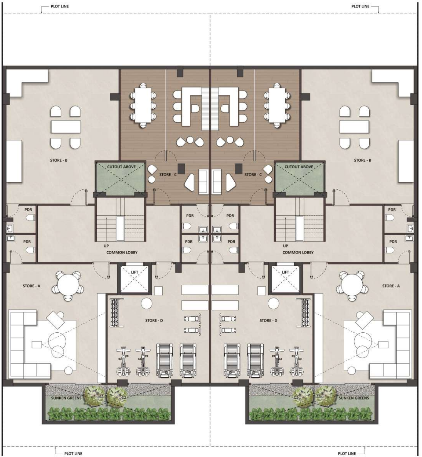
BASEMENT PLAN
