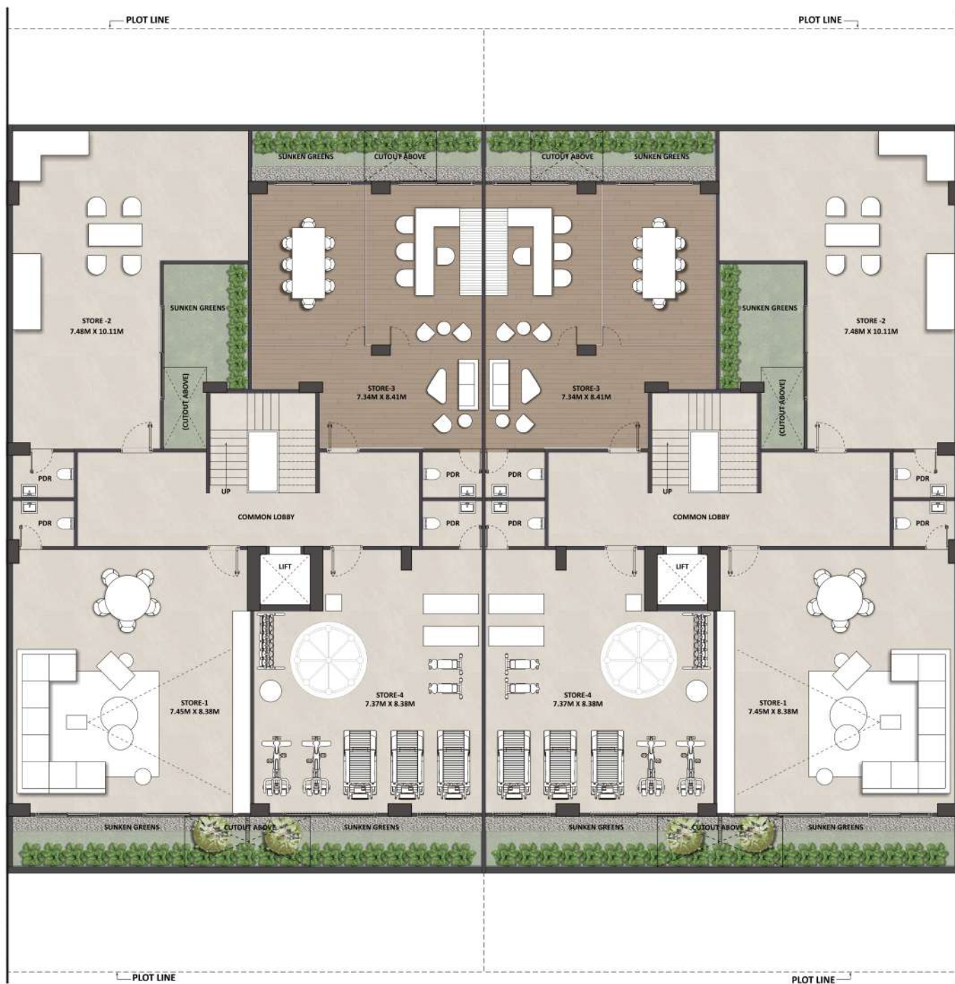
BASEMENT PLAN
